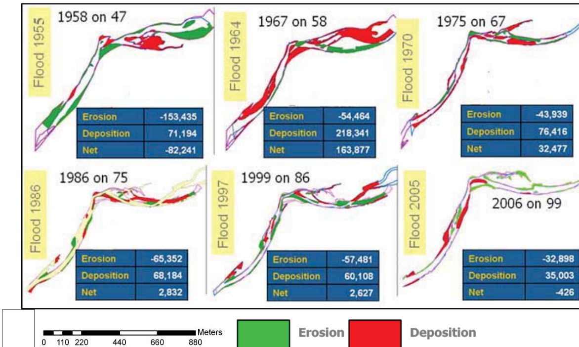
Figure 19. Surface areas of total, bar and terrace, erosion and deposition corresponding to each flood period at the Y3 site. Positive area changes represent deposition; negative area changes are erosion. Values of total erosion and total deposition are for bars plus terraces, while values of bars and terraces represent net changes from erosion plus deposition.
